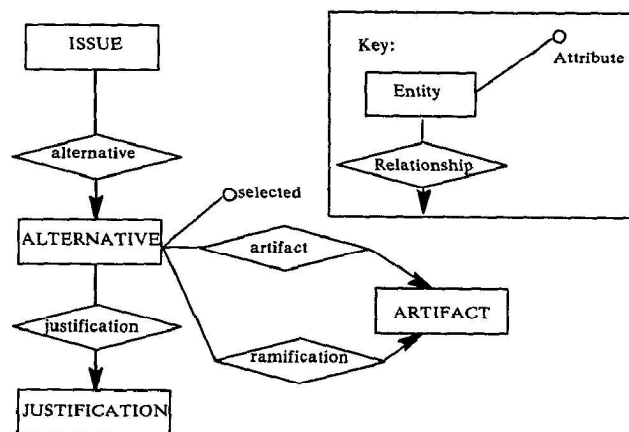
Figure 3: Data model for design deliberation
