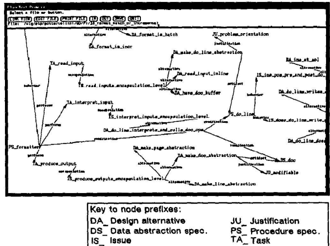
Figure 14: Planetext browser screen for formatter vivisection
