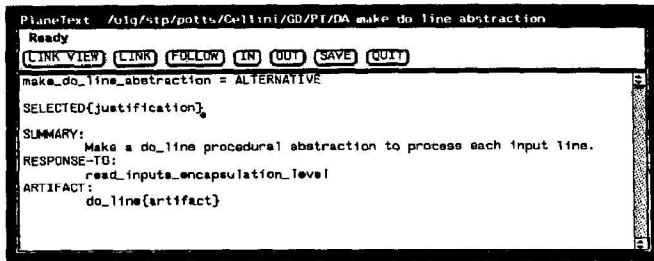
Figure 15: Planetext edit window showing emanating links
