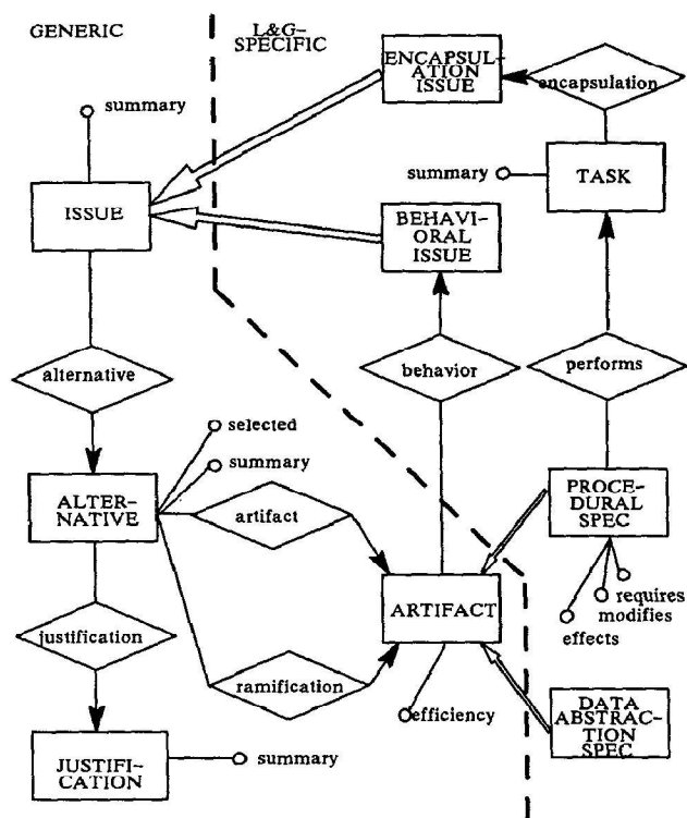
Figure 5: Data model for L&G
